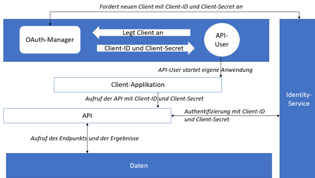
Abb.: OAuth-Client-Workflow
