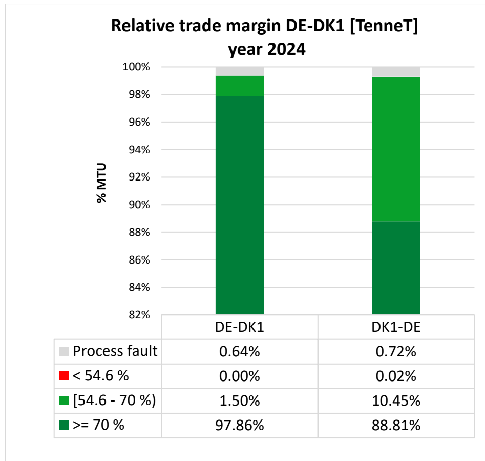
Figure 14: Relative trade margin DE-DK1 [TenneT] year 2024 (minimum value 54.6%)
