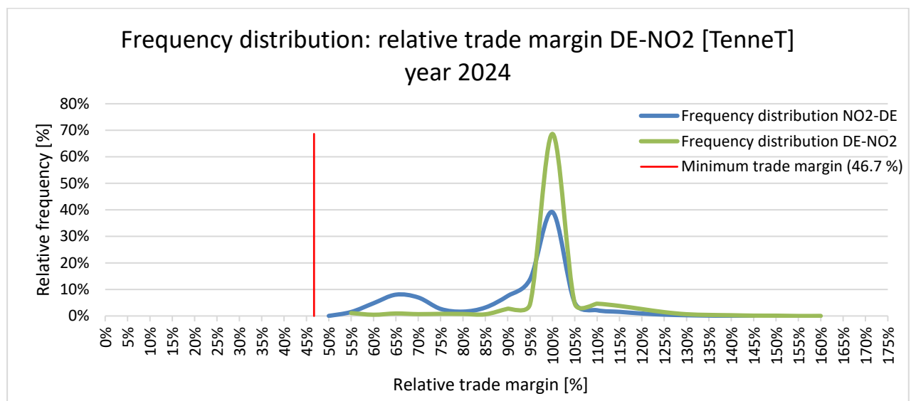
Figure 18: Frequency distribution: relative trade margin DE-NO2 [TenneT] year 2024 (minimum value 46.7%)
