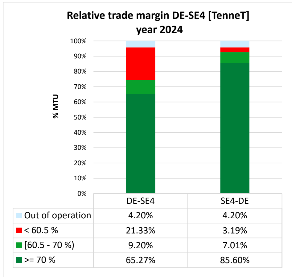
Figure 19: Relative trade margin DE-SE4 [TenneT] 2024 (minimum value 60.5%)
